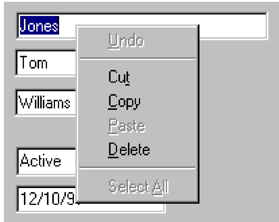
Menu Pop-Up
